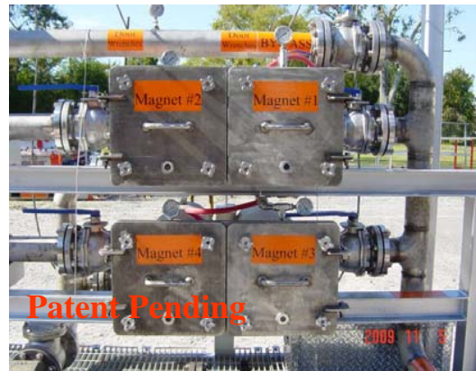
Flow-thru 2 Sets SS Cylinders with Magnets MagneTight™ Rigged-up on Location
