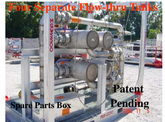
Sight Glass View Magnets & Extra Spare Parts MagneTight™ Flow System—Ready
